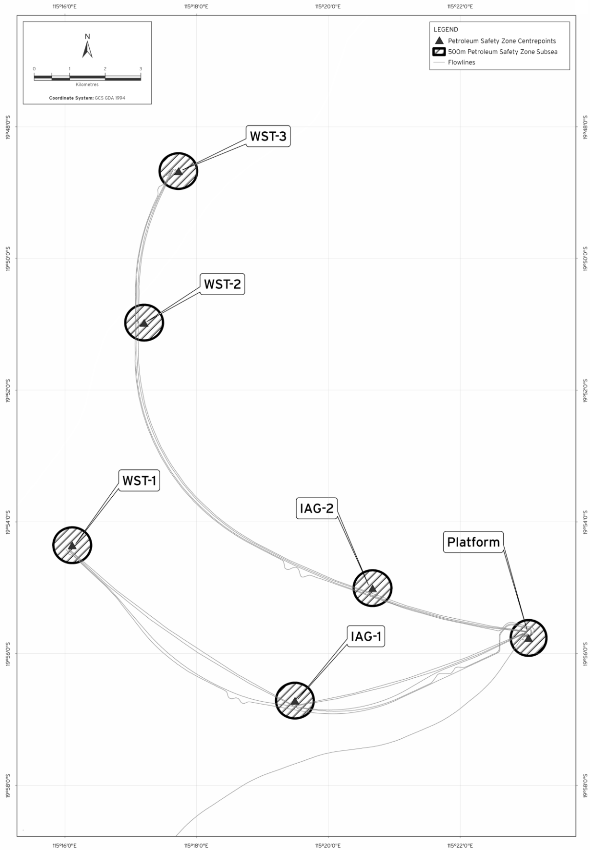
Figure 1 – Diagrammatic representation of petroleum safety zones
