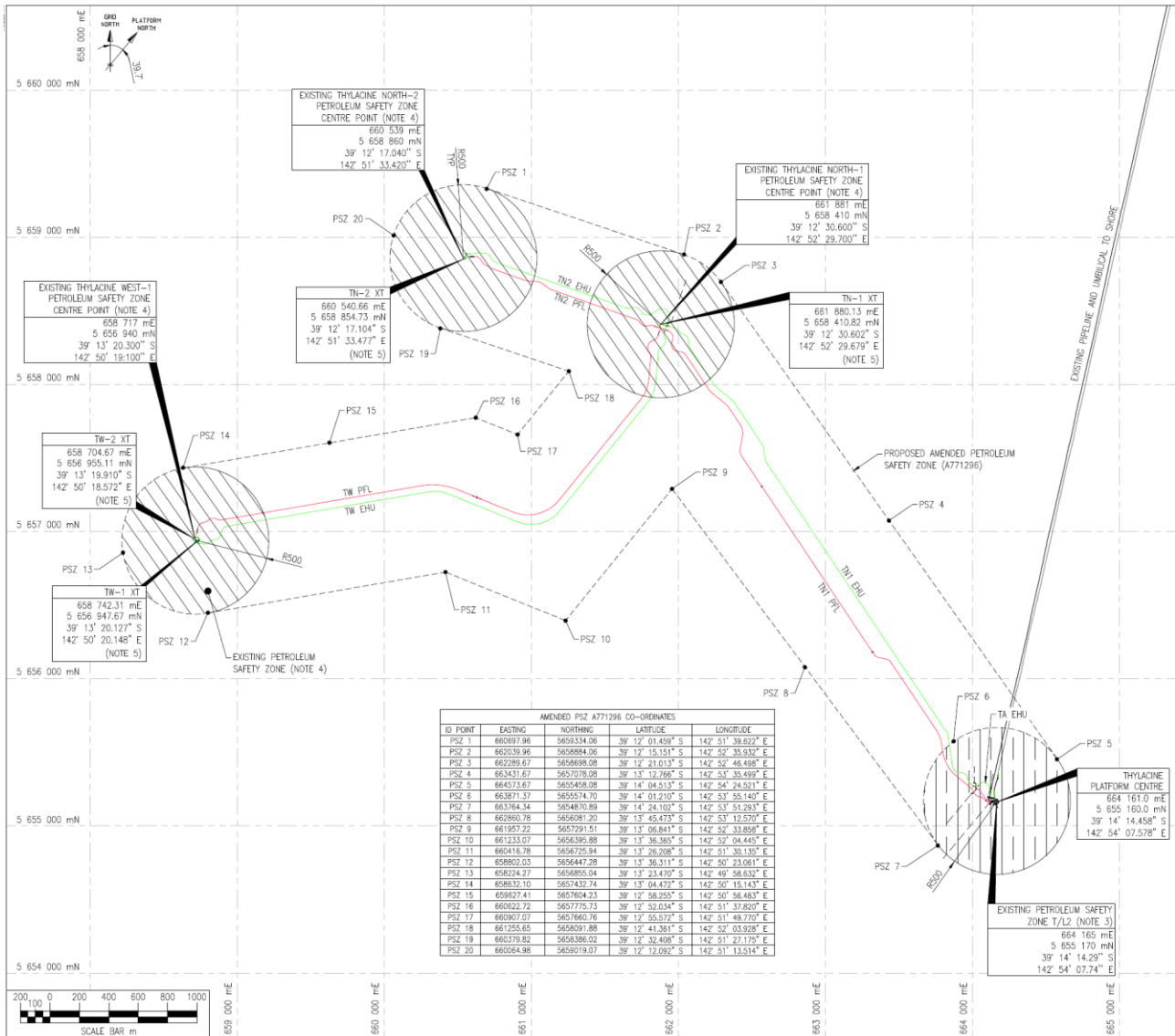
Figure 1 – T/L2 wells, flowlines, umbilicals, and subsea infrastructure Petroleum Safety Zones
