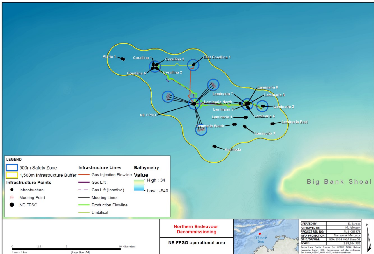
Figure 1 - AC/L5 wells, equipment, and subsea structure Petroleum Safety Zones
